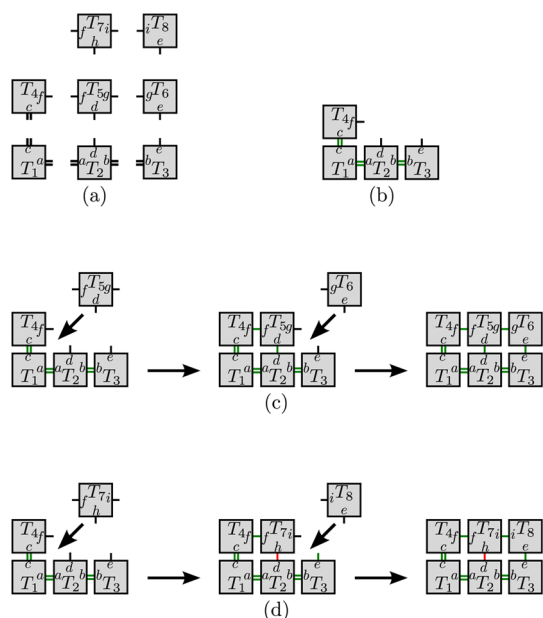
Figure 1. Mechanism of cooperative growth errors. (a) An 8 tile system with a potential for cooperative binding errors in the tile assembly model. 42 Tiles are represented by gray rectangles with face labels. Pad types are shown near the appropriate edge of each tile. Null pads are omitted. Pad strength is indicated by the number of rectangular bars that accompany each pad. Tile system is run at temperature \tau = 2 . (b) Initial error free assembly of 4 tiles. Correctly matched pads are shaded green. (c) Error free assembly pathway to completion from state (b). (d) Erroneous pathway due to cooperative binding error. Mismatched pad highlighted in red.
