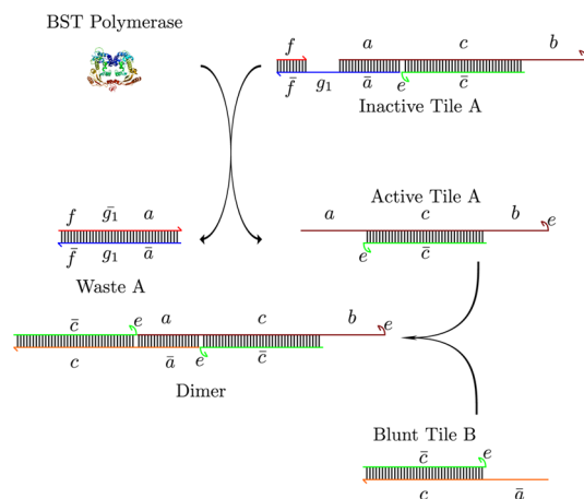
Figure 2. Dimerization of Tile A and Tile B after activation: Inactive Tile A is transformed into Active Tile A by the strand displacing BST DNA Polymerase. Blunt Tile B is a modified version of Active Tile B that lacks the sticky end \bar{b} . This prevents the formation of a linear polymer and assembly is halted after a dimer (Active Tile A and Blunt Tile B) is produced.
