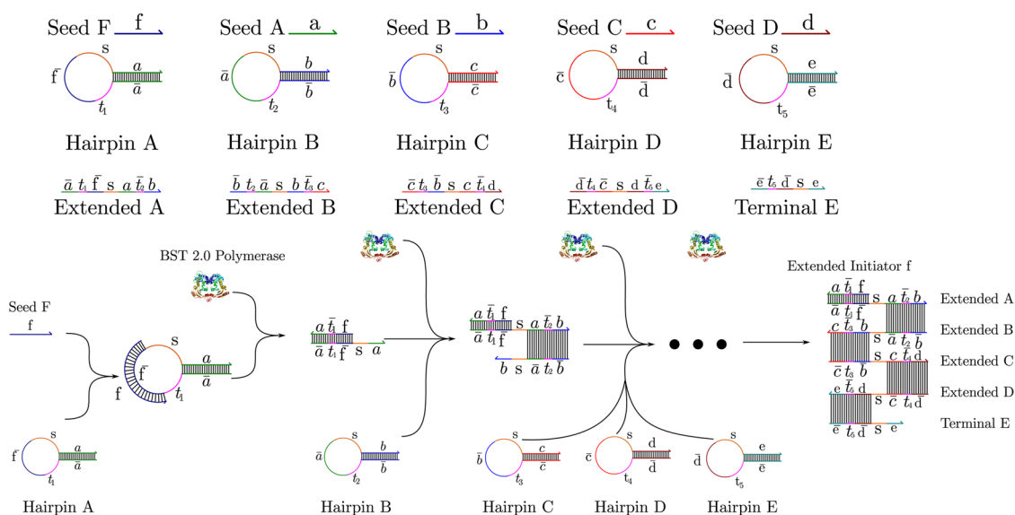
Figure 4. Directed assembly of tiles.
